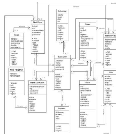
Gambar 5. Class Diagram
